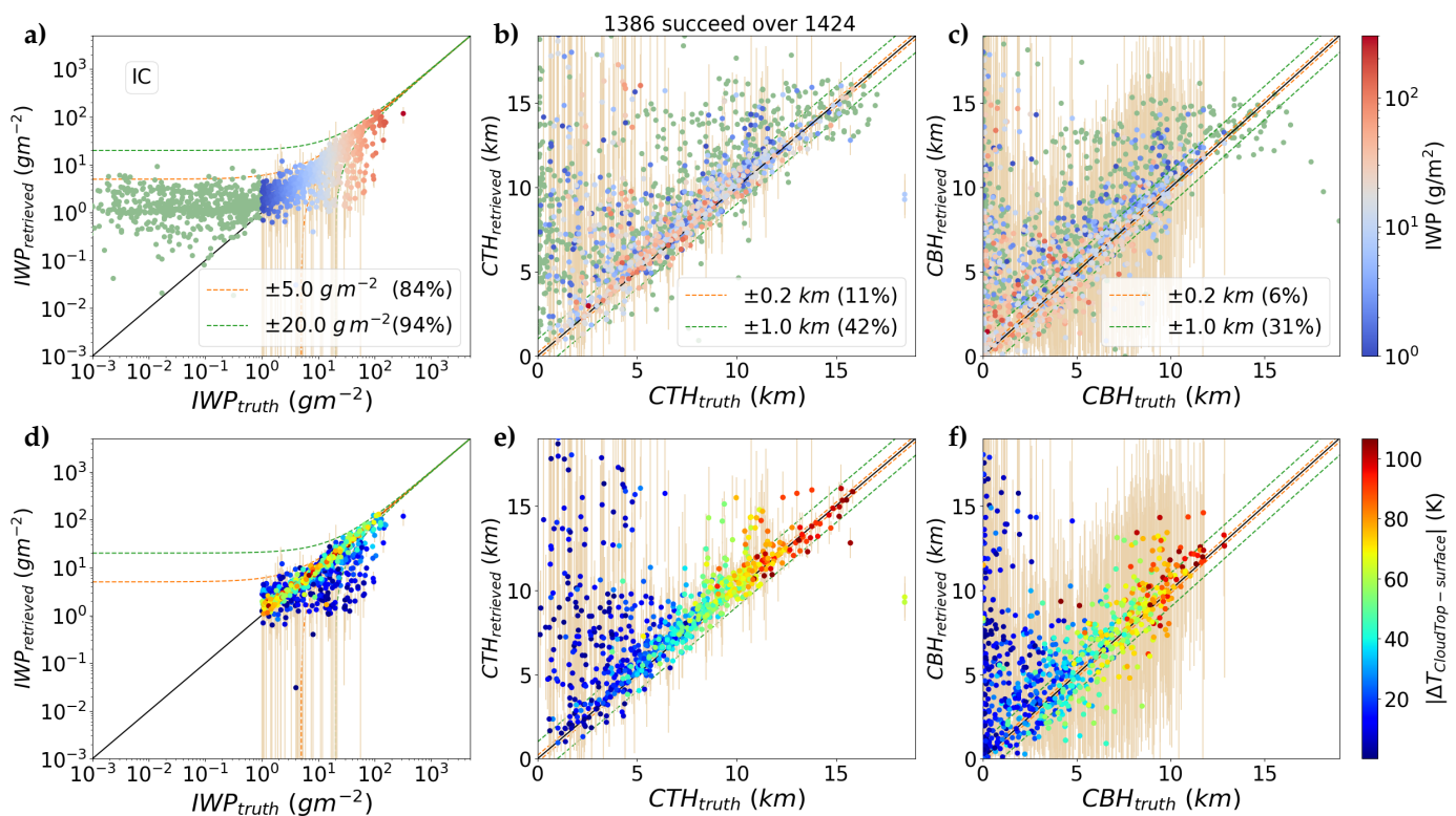
Figure 7. Retrievals of IWP (left, a,d), CTH (center, b,e), and CBH (right, c,f) for IC cloud configuration from IASI synthetic radiances as a function of the true state over all the profile database. In the top panel (a–c), the clouds whose IWP is lower than 1 \text{ g/m}^2 are depicted in green. The color code corresponds to the IWP of the clouds. In the bottom panel (d–f), the clouds whose IWP is lower than 1 \text{ g/m}^2 have been removed. The color code is related to the temperature contrast between the cloud layer and surface. The error bars are plotted in beige. The dotted lines indicate the goal (orange) and threshold (green) given by the World Meteorological Organization in order to reduce uncertainties in weather forecasts. The associated percentage corresponds to the proportion of cases that satisfy the OSCAR goal and threshold.
