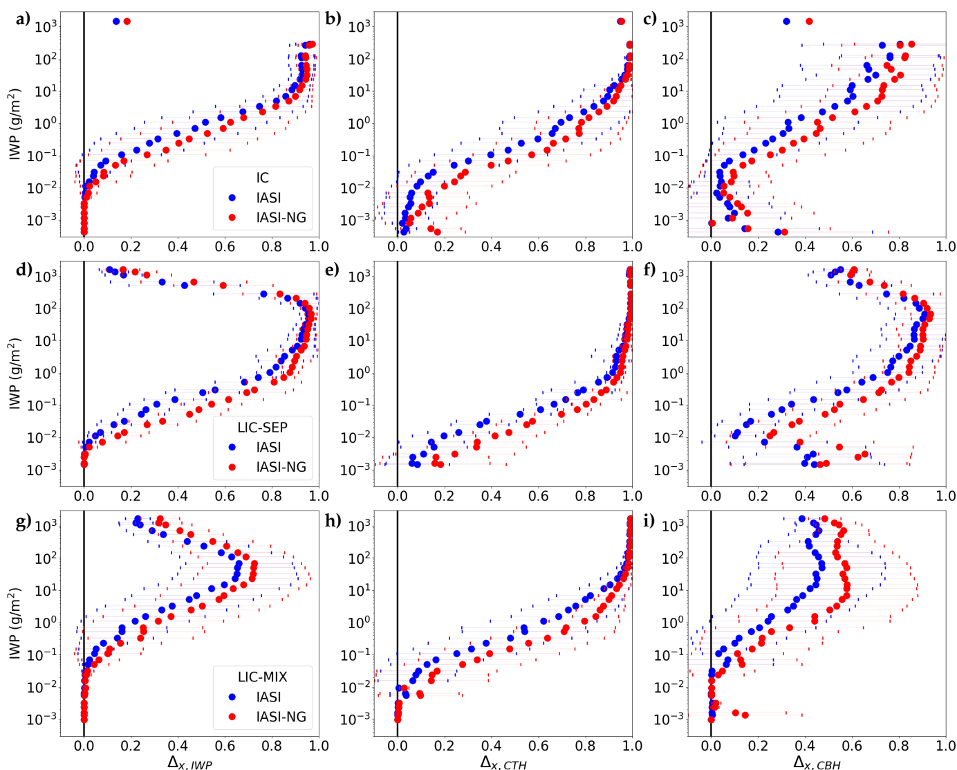
Figure 4. Normalized a priori error departure (difference between the a priori and posterior error normalized by the a priori error) for IWP (left, a,d,g), CTH (center, b,e,h), and CBH (right, c,f,i) for the ice only layer, IC (upper, a–c), separated liquid and ice layers, LIC-SEP (center, d–f), and mixing liquid and ice layers, LIC-MIX (lower, g–i), cloud configurations. The dots stand for the error averaged over IWP bins for the IASI instrumental configuration (in blue) and for IASI-NG (next generation) (red). The x error bars correspond to the standard deviation of the error departure. A value close to 0 implies that the measurement cannot improve our prior knowledge of the parameter. A value close to 1 implies that the parameter can be characterized by the measurement.
