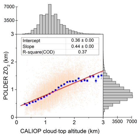
Figure 3. POLDER cloud altitude ( Z_{O_2} ) compared to CALIOP cloud-top altitude, over a period of 6 months (May to October) from 2006 to 2010 along the CALIOP track. Lateral histograms show the data distribution.
