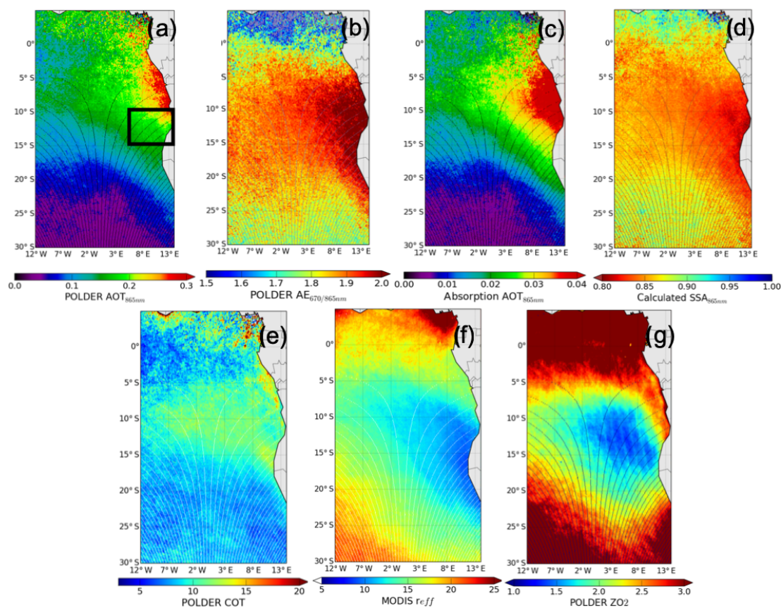
Figure 2. Mean values of above-cloud aerosol and cloud properties above the South Atlantic Ocean, for a period of 6 months (May to October) from 2006 to 2009: (a) POLDER AOT 865 nm . The black box represents the sample area close to Angola’s coast described in Sect. 3.2; (b) POLDER AE 670/865 nm ; (c) POLDER absorption AOT 865 nm ; (d) POLDER SSA 865 nm ; (e) POLDER COT (corrected for above-cloud absorbing aerosols); (f) MODIS effective radius, r_{\text{eff}} ( \mu\text{m} ); (g) POLDER cloud altitude (ZO 2 ) derived from oxygen pressure (km).
