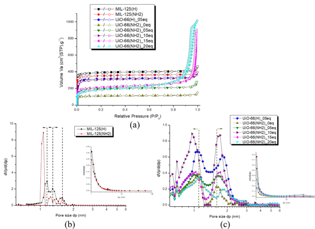
Figure 3: (a) N_2 sorption isotherms and pore size distributions evaluated for (b) MIL-125(X) and (c) UiO-66(X)_Y. The closed and open symbols present in the isotherms refer to the adsorption and desorption branches, respectively.
