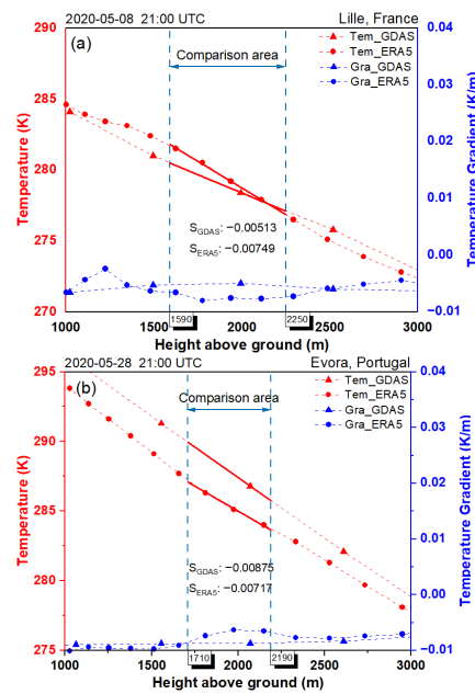
Figure 9. (a) The temperature profiles from Lille: 08 May 2020 21:00 UTC corresponding to the case with the highest deviation of the aerosol extinction shown in Figure 1; (b) The temperature profiles from Evora: 28 May 2020 21:00 UTC corresponding to the case with the lowest deviation of the aerosol extinction shown in Figure 1. Red lines indicate the temperature profiles and blue lines indicate the temperature gradients. The triangle and round shape represent the data from the GDAS and ERA5 models, respectively. The ‘comparison area’ represents the data range used to calculate the deviation, and the S values represent the gradient of the linear fit line of the temperature in the ‘comparison area’ from different models.
