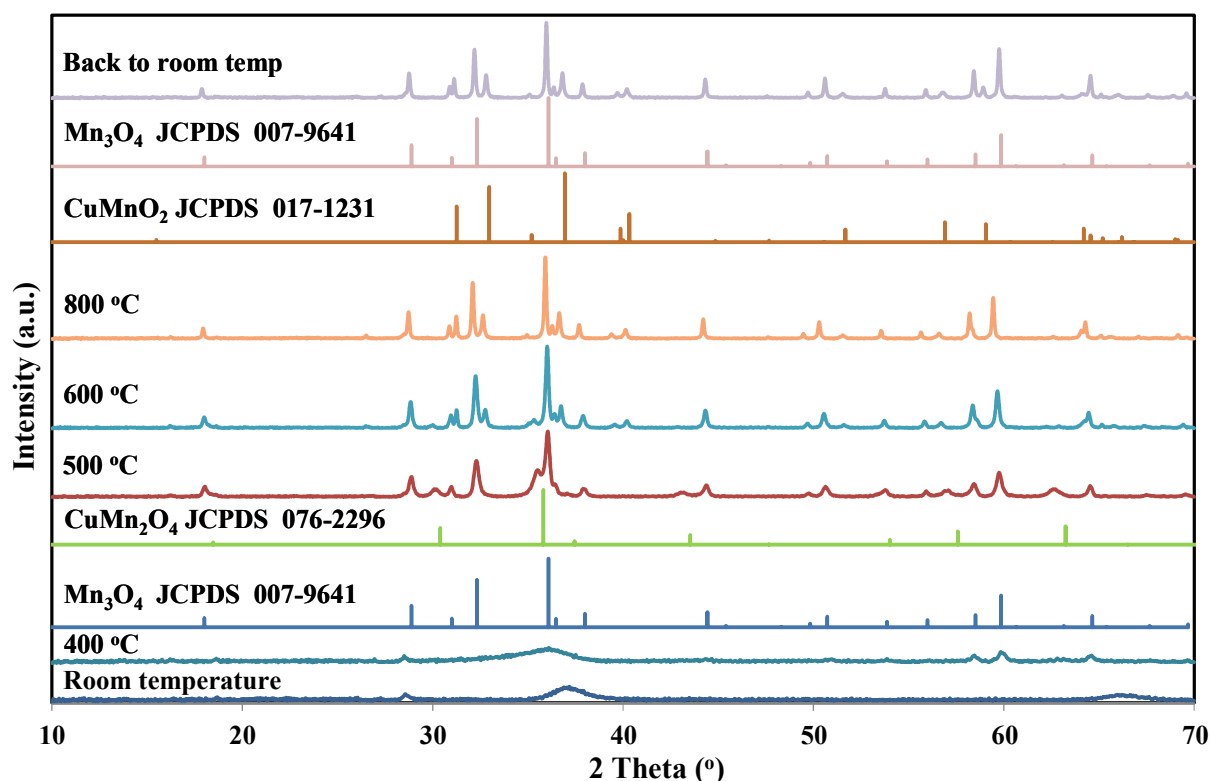
Fig.4: In situ XRD patterns of CuMnOx-R3 under flowing \text{N}_2 as a function of temperature.
