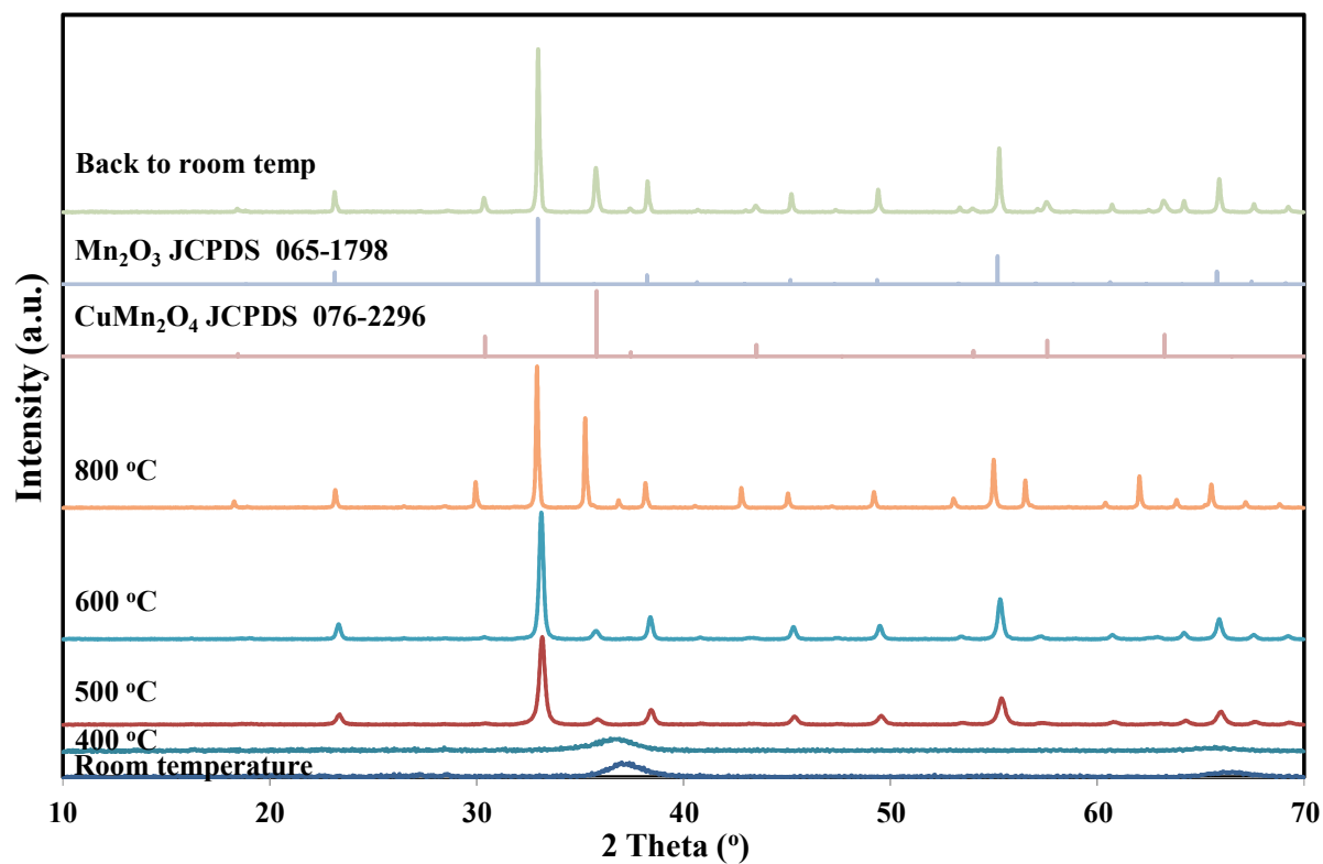
Fig.3: In situ XRD patterns of CuMnOx-R3 under flowing air as a function of temperature.
