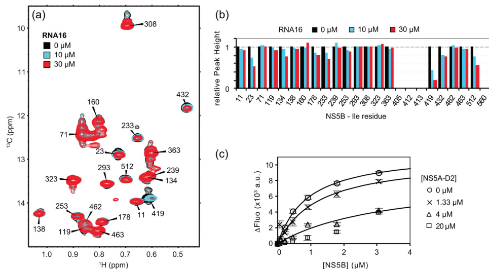
Figure 5. Interaction of NS5B _{\Delta 21} with an RNA oligonucleotide and effect of NS5A-D2. a , superposition of methyl-TROSY spectra of U- ^{15}\text{N} , ^2\text{H} - \delta 1 - ^{13}\text{C} - ^1\text{H}_3 -labeled NS5B _{\Delta 21} (50 \mu\text{M} ) recorded in the presence of increasing concentrations (0, 10, and 30 \mu\text{M} ) of RNA16. b , ratios of peak heights of Ile methyl ( \delta 1 ) resonances in methyl-TROSY spectra of NS5B _{\Delta 21} obtained in the presence and absence of different concentrations of RNA16. Peak heights in individual spectra were first normalized to that of the invariant Ile-293 resonance to correct for the observed sample precipitation over the course of the titration. c , titration of a fluorescent RNA oligonucleotide (6FAM-RNA16, 50 nM) with increasing concentrations of NS5B _{\Delta 21} . The increase in fluorescence intensity (515–525 nm) of 6FAM-RNA16 is plotted as a function of NS5B _{\Delta 21} concentration. The titration experiment was performed in the absence and in the presence of NS5A-D2 (0, 1.33, 4, and 20 \mu\text{M} ). Error bars, one S.D. value of three replicates. Corresponding dissociation constants were obtained by fitting the experimental data to the theoretical equation corresponding to a reversible complex.
