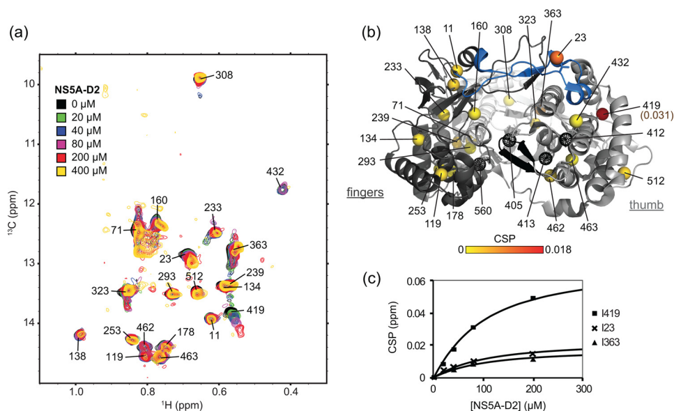
Figure 3. NS5A-D2 interacts with NS5B Δ21 . a , superposition of methyl-TROSY spectra of U- 15 N, 2 H 3 -Ile δ 1 - 13 C 1 H 3 -labeled NS5B Δ21 (40 μM) recorded in the presence of increasing concentrations (0, 20, 40, 80, 200, and 400 μM) of unlabeled NS5A-D2. b , 1 H, 13 C combined CSPs observed in the NS5B–NS5A-D2 (1:2 molar ratio) in a spectrum mapped, from yellow (0 ppm) to red (0.018 ppm), onto the Ile δ 1 methyl groups of the NS5B structure (PDB code 2XXD). The CSP for Ile-419 is 0.031 ppm (above the defined upper limit) and is highlighted. Methyl groups that were not observed are shown as black dotted spheres. The figure was prepared using PyMOL. c , titration curves corresponding to the experiments in a . 1 H, 13 C combined CSPs observed for Ile-419, Ile-23, and Ile-363 residues in NS5B Δ21 are plotted as a function of increasing concentrations of NS5A-D2. Corresponding dissociation constants were obtained by fitting the experimental data to the theoretical equation corresponding to a reversible complex.
