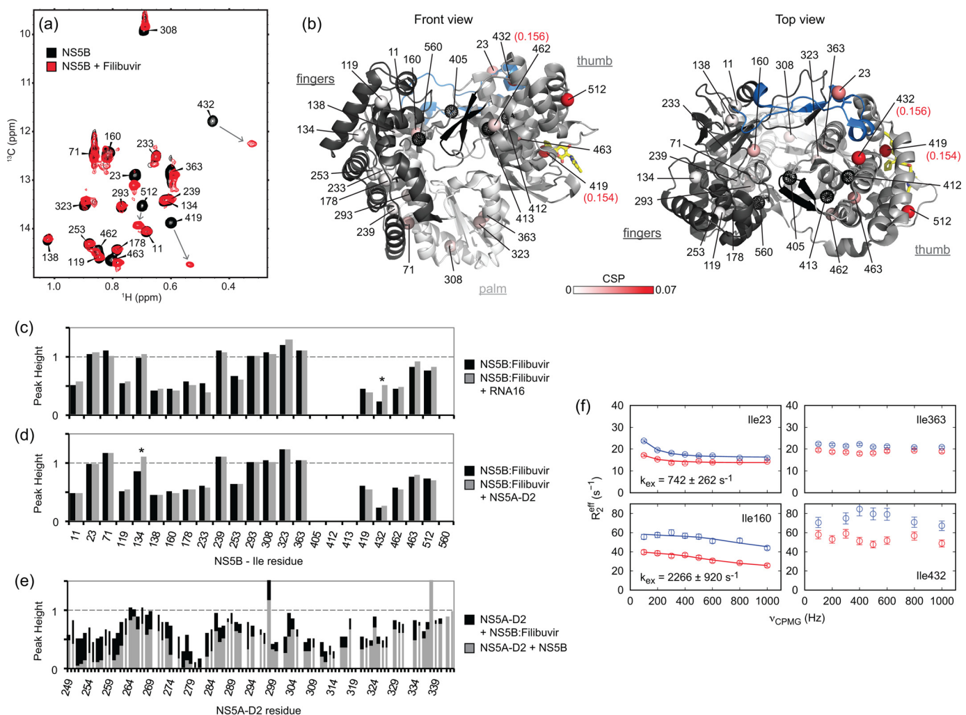
Figure 7. N55B and its inhibition by filibuvir. a , superposition of methyl-TROSY spectra of N55B _{\Delta 21} (in black) and the N55B _{\Delta 21} -filibuvir complex (in red). b , ^1\text{H} , ^{13}\text{C} combined CSPs following filibuvir binding are mapped, from white (0 ppm) to red (0.07 ppm), onto the Ile methyl groups of the N55B structure (PDB code 2XXD). CSPs for Ile-419 and Ile-432 are 0.154 and 0.156 ppm (above the defined upper limit) and are highlighted. Methyl groups that were not observed are depicted as black dotted spheres. Figures were prepared using PyMOL. c , effect of filibuvir on the N55B interaction with RNA16. Relative peak heights of Ile methyl ( \delta 1 ) resonances in ^1\text{H} , ^{13}\text{C} TROSY spectra of the N55B _{\Delta 21} -filibuvir complex (50 \mu\text{M} ) obtained in the absence and in the presence of RNA16 (30 \mu\text{M} ) are shown. For each spectrum, peak intensities are normalized to the Ile-293 signal. d and e , effect of filibuvir on the N55B interaction with NS5A-D2. d , relative peak heights of Ile methyl ( \delta 1 ) resonances in ^1\text{H} , ^{13}\text{C} TROSY spectra of the N55B _{\Delta 21} -filibuvir complex (50 \mu\text{M} ) obtained in the absence and in the presence of NS5A-D2 (50 \mu\text{M} ) are shown. For each spectrum, peak intensities are normalized to the Ile-293 signal. e , relative peak heights of backbone amide resonances in ^1\text{H} , ^{15}\text{N} HSQC spectra of ^{15}\text{N} -labeled NS5A-D2 (20 \mu\text{M} ) in the presence of unlabeled N55B _{\Delta 21} (100 \mu\text{M} ; gray bars) or unlabeled N55B _{\Delta 21} -filibuvir complex (100 \mu\text{M} ; black bars), normalized to peak heights in the absence of N55B. f , methyl-TROSY MQ CPMG relaxation dispersion data for N55B _{\Delta 21} Ile residues 23 (fingertips), 160 (fingers), 363 (palm), and 432 (thumb) in the presence of filibuvir. Red, 600 MHz; blue, 900 MHz. For residues 23 and 160 exhibiting non-flat dispersion curves, exchange rates ( k_{\text{ex}} ) fitted individually are indicated in the panels. Fits were performed allowing only ^{13}\text{C} \Delta\omega to vary.
