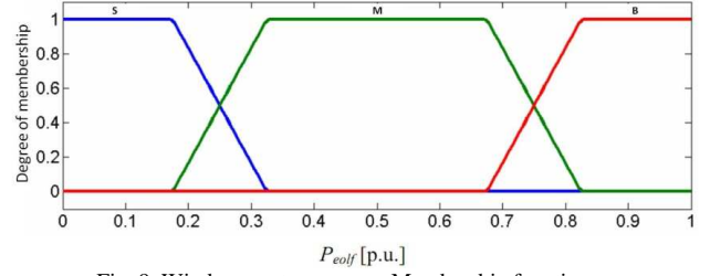
Fig. 9. Wind generator power – Membership functions.
