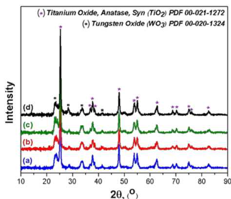
Fig. 1. Powder XRD patterns recorded on W/T (a); VW/T (b); VW/T-K2 (c); WV/T-K8 (d) calcined in air at 450°C
