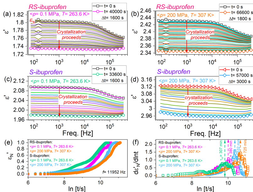
Figure 3. Time evolutions of the dielectric \epsilon' spectra for RS-ibuprofen (a and b) and S-ibuprofen (c and d) during the isothermal crystallization measurements. Results obtained for RS-ibuprofen and S-ibuprofen under the same condition of p = 0.1 MPa, T = 263.6 K are depicted in panels (a) and (c), respectively. Panels (b) and (d) show the results for RS-ibuprofen and S-ibuprofen recorded under the same conditions of p = 200 MPa, T = 307 K. Panel (e): relations of \epsilon'_N - \ln t for the tested S-ibuprofen and RS-ibuprofen samples. The results are ascertained at a fixed frequency of 11 952 Hz. Panel (f): time dependences of the first derivative of \epsilon'_N against the natural logarithm of time ( d\epsilon'_N/d \ln t ) in terms of the Avramov approach.
