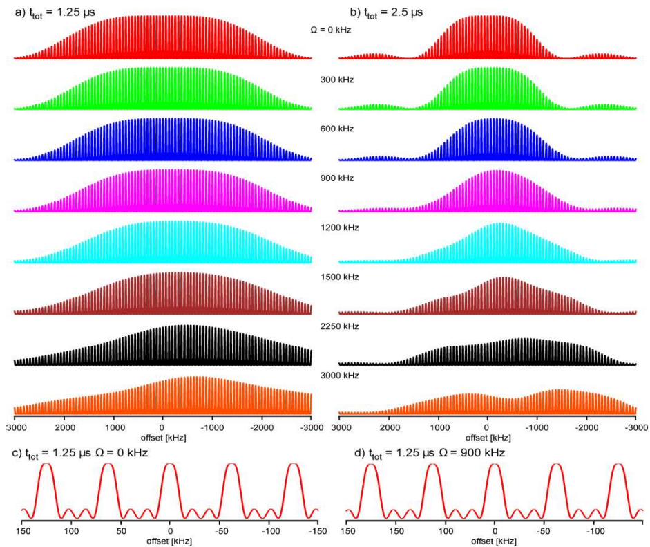
Fig.7. Simulated envelope efficiency of ^1\text{H}\{-^{195}\text{Pt}\} D-HMQC experiments with D_1^4 excitation with (\nu_1(\text{kHz}), t_{\text{tot}}(\mu\text{s})) = (200, 1.25) (a) or (100, 2.5) (b), versus ^{195}\text{Pt} offset for 8 CSA span values ranging from \Omega = 0 -3000 kHz. (c,d) Expansions showing the individual rf-spikelets, which are CSA and rf independent (Eq.1).
