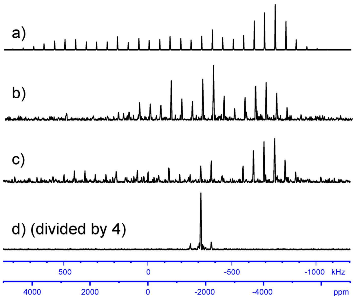
Fig.14. Cisplatin MAS spectra at 18.8 T with \nu_R = 62.5 kHz. (a) 1D spectrum simulated after a Dirac single pulse. (b-d) projections onto the ^{195}\text{Pt} axis of ^1\text{H}\{-^{195}\text{Pt}\} D-HMQC 2D constant-time spectra ( 2nT_R = 0.176\text{ms} [23]) with ^{195}\text{Pt} on-resonance excitation, recorded with SR4 1 2 : m = 32 , \tau_{RD} = 0.8 s, NS = 64, 512 complex t_1 points, \Delta t_1 = 0.4 \mu\text{s} (SW1 = 2.5 MHz), T_{\text{exp}} = 13\text{h} . ^{195}\text{Pt} excitation with (\nu_1 (kHz), t_p/t_{\text{tot}} ( \mu\text{s} )) = (200, 1.25) HP (b) or D 1 4 (c) or (42, 24) SLP (d).
