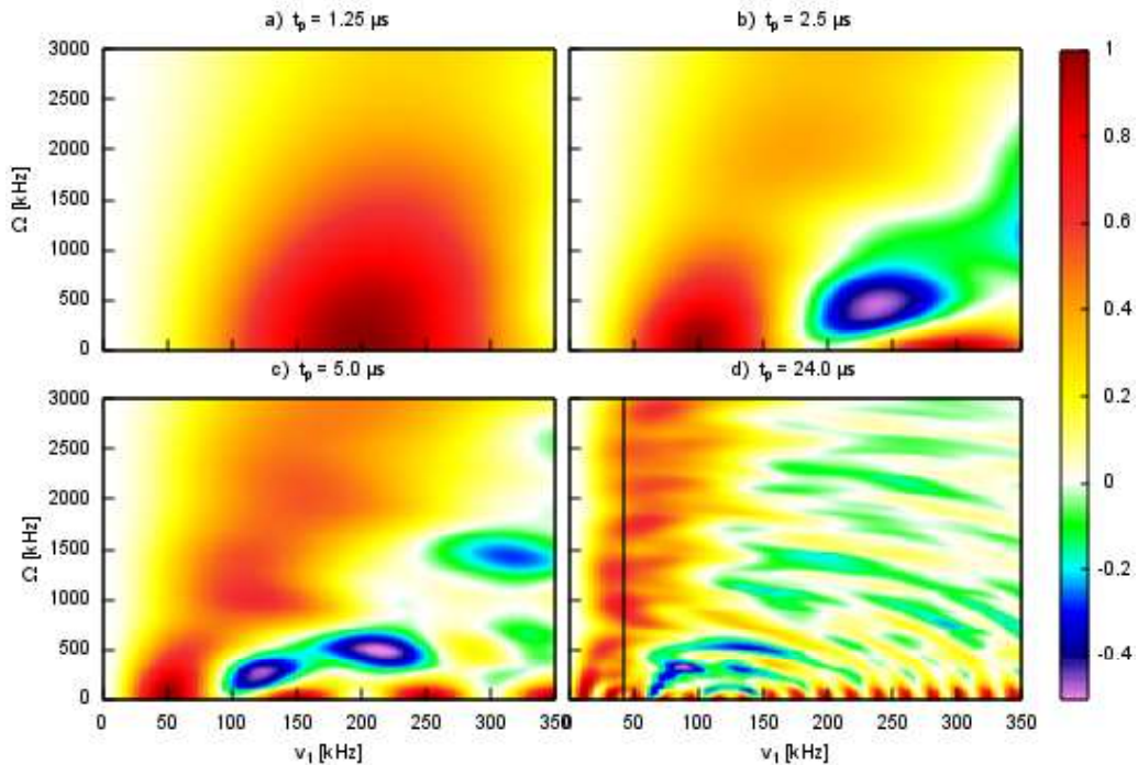
Fig.3. Simulated on-resonance efficiency of ^1\text{H}\{-^{195}\text{Pt}\} D-HMQC experiments versus ( \nu_1 & \Omega ) for four typical t_p pulse durations, as indicated of the subfigures. In (d), the condition \nu_1 = 2\nu_R/3 = 42 kHz is indicated by a black vertical line.
