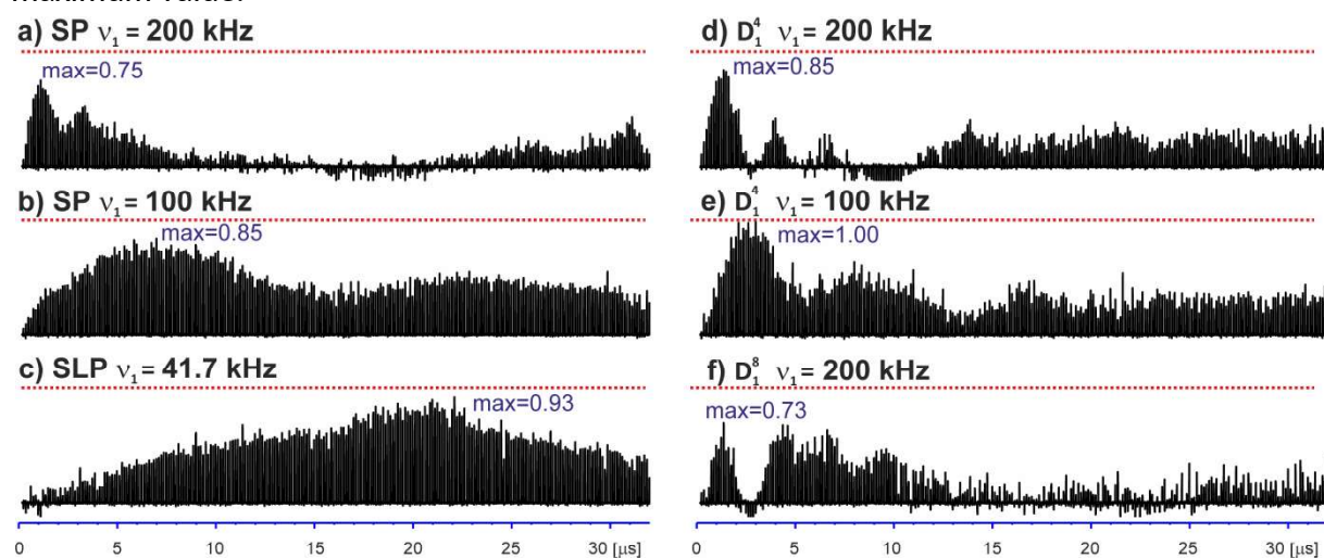
Fig.10. Experimental cisplatin ^1\text{H}\{-^{195}\text{Pt}\} rotor-synchronized D -HMQC on-resonance 1D ^1\text{H} signal with \tau_{\text{RD}} = 13 s and NS = 16, versus the pulse length on ^{195}\text{Pt} : t_p (SP) or t_{\text{tot}} = kt_p ( D_1^k ), with \nu_1 = 200 (a,d,f), 100 (b,e), 42 kHz (c).
