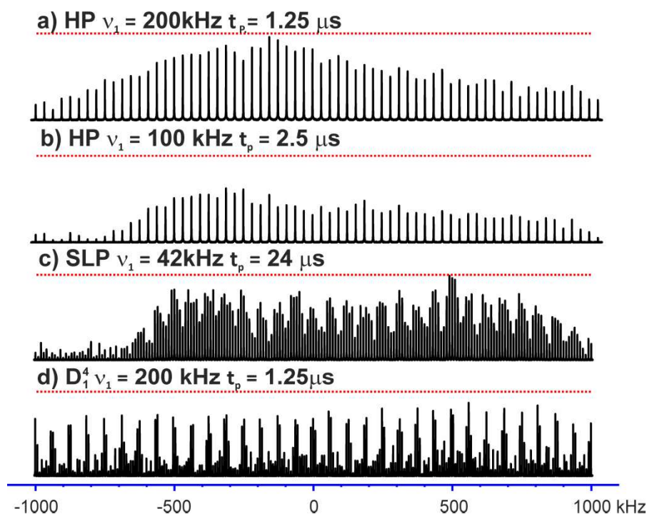
Fig.11. Experimental cisplatin ^1\text{H}\{-^{195}\text{Pt}\} rotor-synchronized D-HMQC ^1\text{H} signal with \tau_{\text{RD}} = 13 s and NS = 16 versus the ^{195}\text{Pt} offset, with various types of excitation, rf-field and pulse length ( t_p or t_{\text{tot}} ) as indicated on the subfigures. The offset step is equal to v_R/2 = 31.25 (a,b), 10 (c) and 8 kHz (d). It must be noted that in (b) the pulse length does not correspond to the optimum intermediate regime (Fig.10b).
