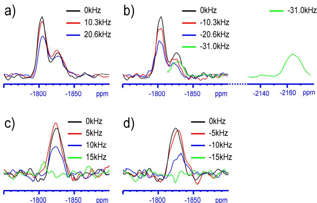
Fig.12. Experimental ^{195}\text{Pt} projections of ^1\text{H}\{-^{195}\text{Pt}\} rotor-synchronized D -HMQC 2D spectra recorded at 18.8 T with \nu_R = 62.5 kHz, \tau_{\text{RD}} = 1 s, 64 complex t_1 points, NS = 64, and T_{\text{exp}} = 2.5 hrs, versus the position of the ^{195}\text{Pt} carrier frequency. (a,b) SLP excitation ( \nu_1 = 42 kHz, t_p = 24 \mu\text{s} ) of a cis- and transplatin mixture with \nu_{\text{offset}} = 0, \pm 10.33, \pm 20.66, -31 kHz. (c,d) D_1^4 excitation ( \nu_1 = 200 kHz, t_{\text{tot}} = 1.25 \mu\text{s} ) of cisplatin with \nu_{\text{offset}} = 0, \pm 5, \pm 10, \pm 15 kHz. The carrier frequency is defined with respect to: (a,b) the middle of the two signals (-1817 ppm), (c,d) the on resonance signal (-1828 ppm).
