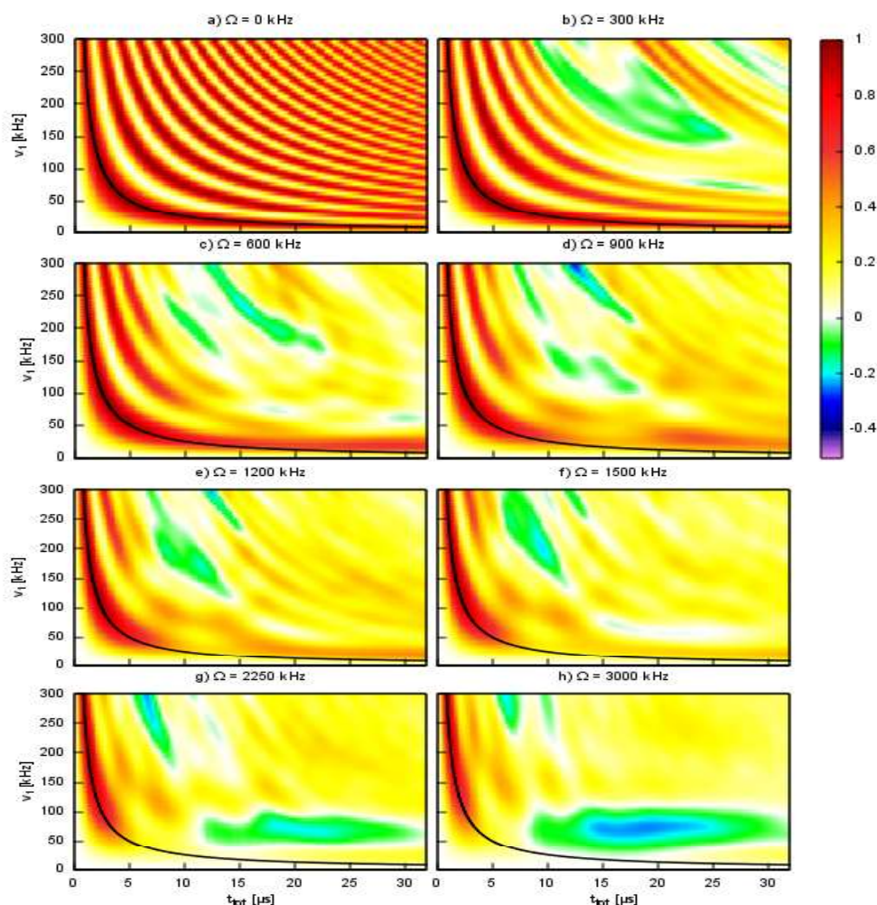
Fig.6. Simulated efficiency of ^1\text{H}\{-^{195}\text{Pt}\} D-HMQC experiments with D_1^4 excitation versus the rf-field strength and the total pulse duration ( t_{\text{tot}} = 4t_p ), for eight CSA values, as indicated. On each sub-figure, the black curve represents the behavior for two \pi/2 -HPs.
