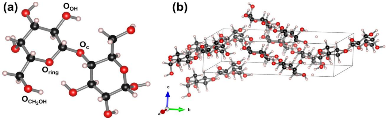
Figure 5. Ball-and-stick representation of a gas-phase molecule \alpha -Lactose (a) and the hygroscopic \alpha -Lactose molecular crystal (b). The unit cell of the latter is indicated with a box. The different O sites are indicated in the gas-phase molecule.
