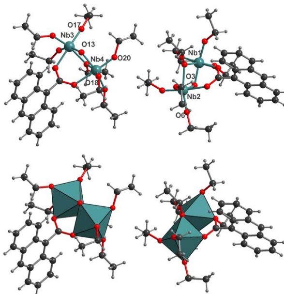
Figure 5: Ball and stick (top) and polyhedral (bottom) representations of the molecular coordination complex 5 . For one molecule, one of the ethoxy groups linked to Nb2 site (through Nb2-O6 bonding) is disordered on two equivalent positions. The same configuration occurs for the Nb3 and Nb4 sites of the second molecule with three disordered ethoxy groups (through Nb3-O17, Nb4-O18 and Nb4-O20 bondings). Only one of these ethoxy groups is shown for clarity.
