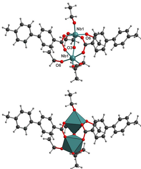
Figure 4: Ball and stick (top) and polyhedral (bottom) representations of the molecular dinuclear coordination complex 4 . One of the ethoxy groups linked to Nb1 site (through Nb1-O6 bonding) is disordered on two equivalent positions. Only one of these ethoxy groups is shown for clarity.
