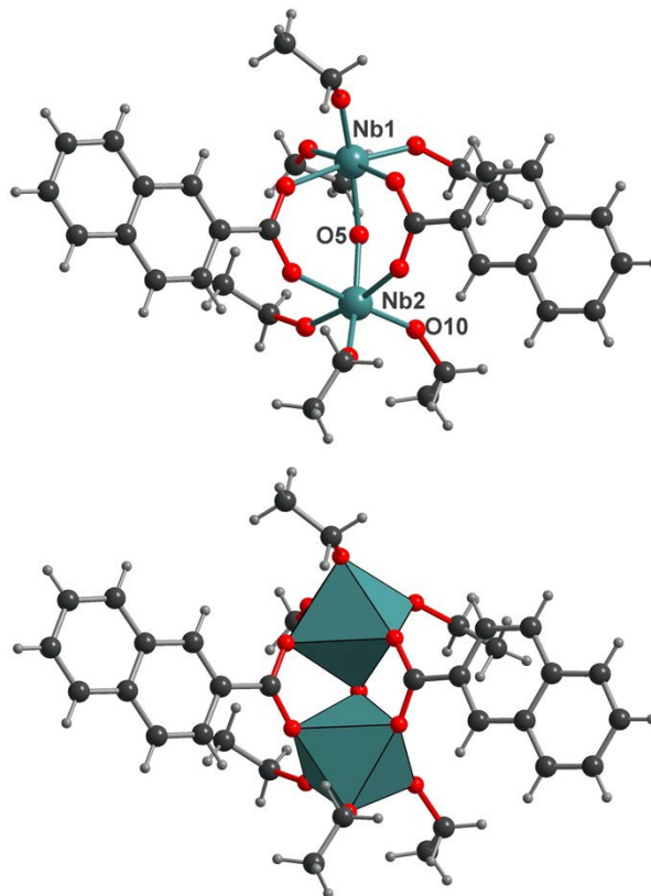
Figure 2: Ball and stick (top) and polyhedral (bottom) representations of the molecular dinuclear coordination complex 2 . One of the ethoxy groups linked to Nb2 site (through Nb2-O10 bonding) is disordered on two equivalent positions. Only one of these ethoxy groups is shown for clarity.
