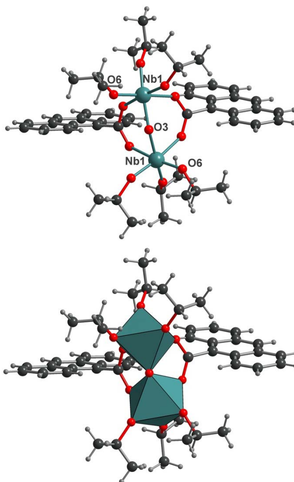
Figure 6: Ball and stick (top) and polyhedral (bottom) representations of the molecular dinuclear coordination complex 6 . One of the isopropoxy groups linked to Nb1 site (through Nb1-O6 bonding) is disordered on two equivalent positions. For them, the methyl groups is located on two close equivalent positions with occupancy 53/47. Only two of the four methyl groups are shown for clarity.
