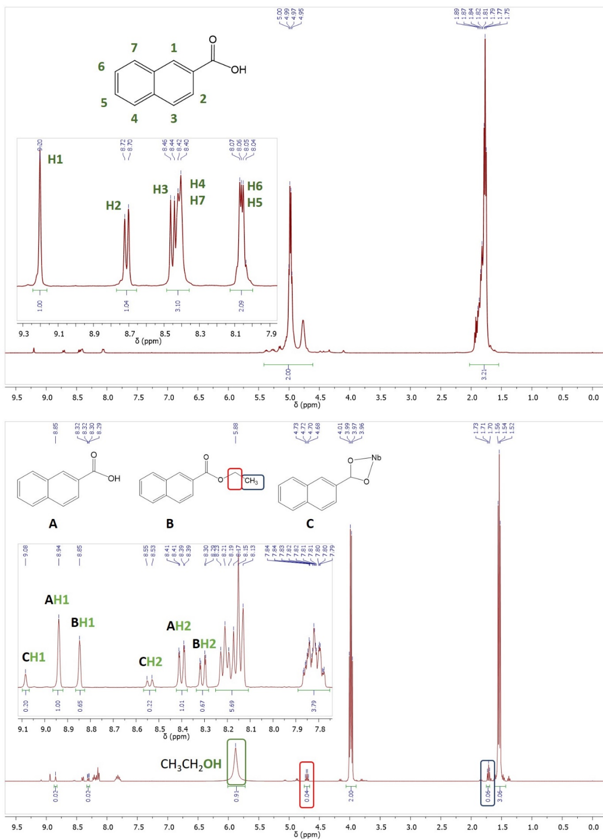
Figure 9: 1 H NMR spectra focused in the aromatic region for the supernatant of complex 2 before (top) and after the crystallization (bottom) with a focus in the aromatic region. With green box: hydroxylic proton of ethanol, red box: -CH 2 group of ester form B and blue box: -CH 3 group of ester form B.
