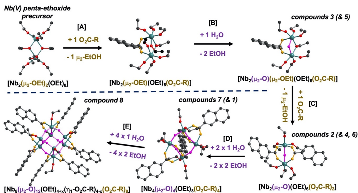
Figure 11: Schematic proposed reaction pathways for the formation of dinuclear, tetranuclear and octanuclear cores of niobium(V) monocarboxylates coordination complexes 1-8 . For compound 8 , only bidentate 2-naphthoate linkers are shown; terminal monodentate 2-naphthoate ligand are not shown for clarity. Green: niobium; dark grey: carbon; red: oxygen from ethoxy group; purple: bridging oxygen between Nb centers; orange: oxygen from bidentate carboxylate groups.
