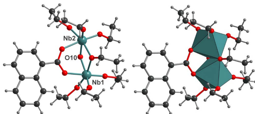
Figure 3: Ball and stick (top) and polyhedral (bottom) representations of the molecular dinuclear coordination complex 3 .
