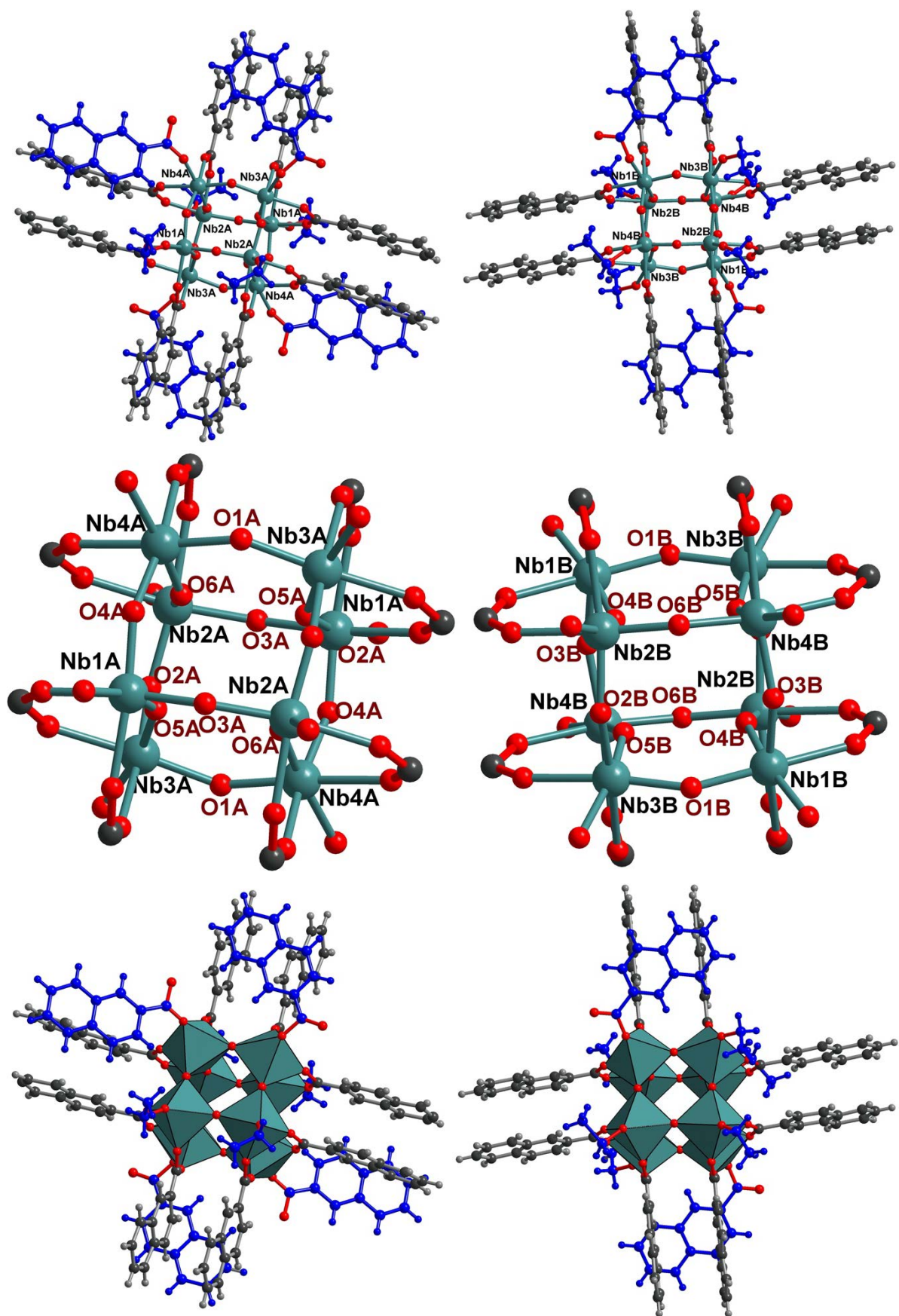
Figure 8: Ball and stick (top) and polyhedral (bottom) representations of the molecular octanuclear coordination complex 8 . The latter consists of two distinct inequivalent entities which contains either 4 ethoxy groups / 4 monodentate 2-naphthoate groups (Molecule A - left) or 6 ethoxy groups / 2 monodentate 2-naphthoate groups
