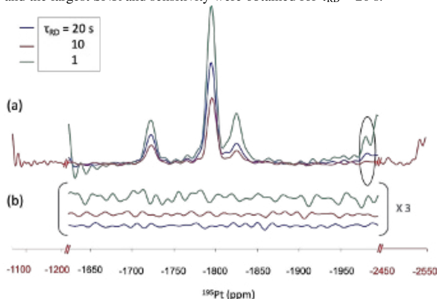
Fig.13. 1D F_1 slices at \delta_{IH} = 4 (a) or 32 (b) ppm of the 2D ^1\text{H}\{-^{195}\text{Pt}\} T-HMQC spectra shown in Figs.12 and 14 of an aged mixture of cis- and transplatin recorded at 18.8 T with \nu_R = 64 kHz and \delta_{\text{off}} = -1810 ppm. The thermal noise has been scaled up by a factor of three in (b). The red slice in (a) is extracted from the 2D spectrum of Fig.14a with SW_1 = 4\nu_R , and hence, additional regions corresponding to the edges of the spectra are also displayed to show the axial peaks. The oval indicates the region containing the impurity signal at -1990 ppm.
