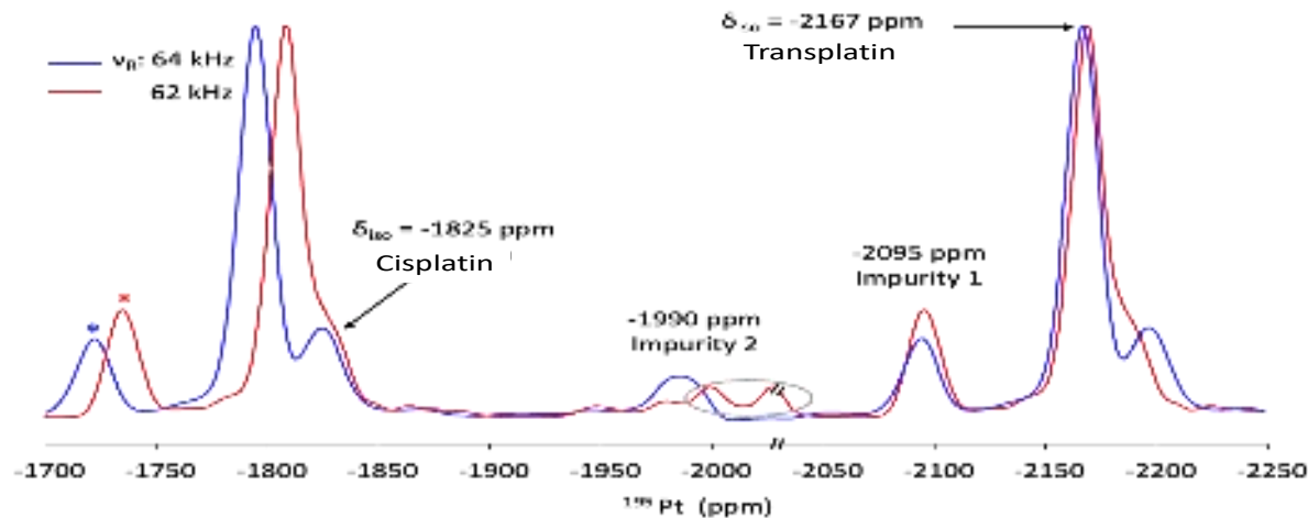
Fig.15. 1D F_1 slices at \delta_{\text{IH}} = 4 ppm duplicated over 2\nu_R of the 2D ^1\text{H}\{-^{195}\text{Pt}\} T-HMQC spectra shown in Figs.12a and 14b of an aged mixture of cis- and transplatin recorded at 18.8 T with \nu_R = 64 and 62 kHz and \delta_{\text{off}} = -1810 or -1850 ppm, respectively. The centerbands are identified by their \delta_{\text{iso}} values, and the symbol * denotes the spinning sidebands. The oval indicates the axial peak on the edge of the spectrum.
