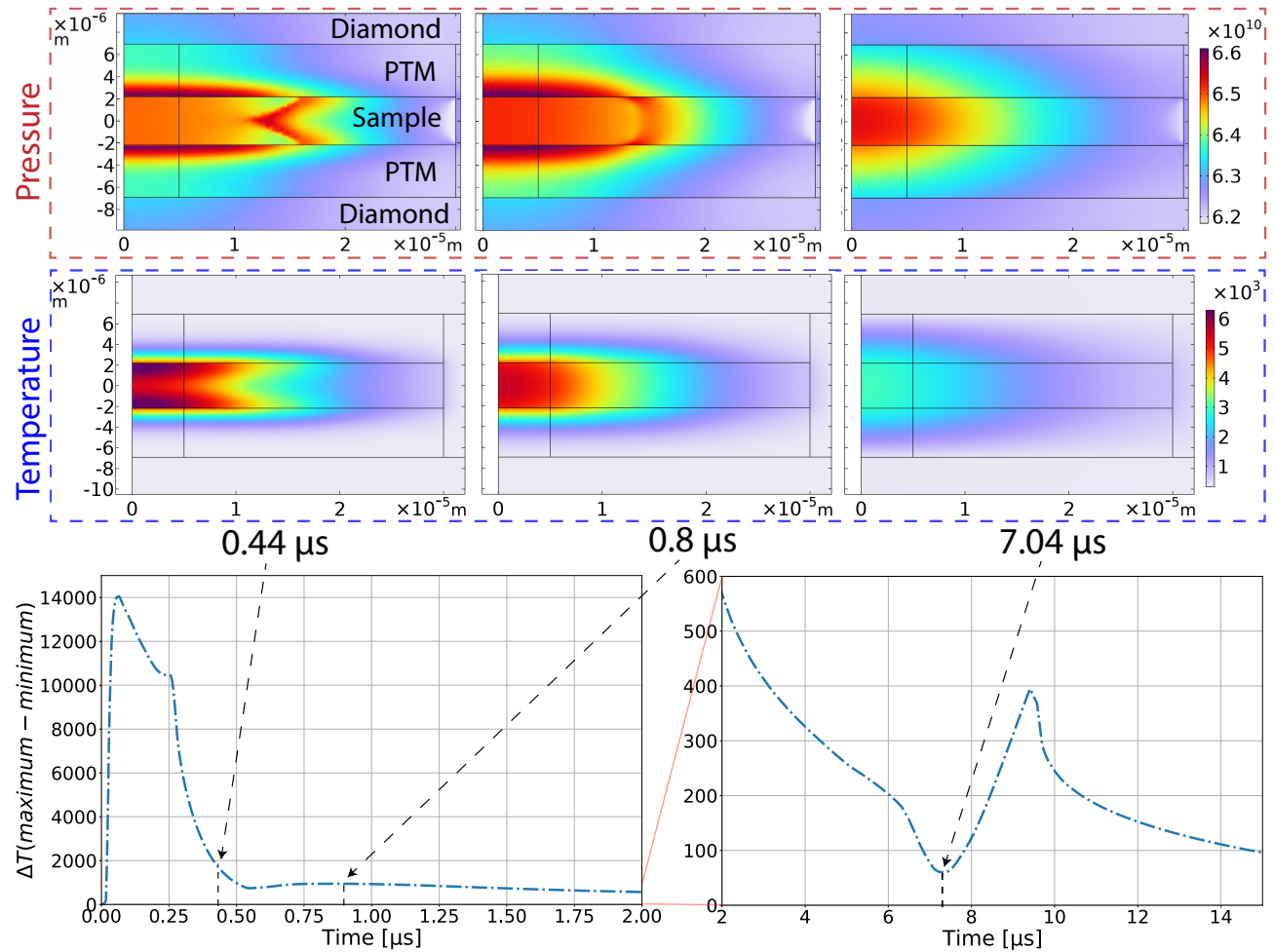
FIG. 14. Top and middle three figures respectively model's total pressure ( P_{ref} + P_{th} ) and temperature maps at t=0.44 \mu\text{s} , 0.8 \mu\text{s} and 7.04 \mu\text{s} (from left to right). For the model reproducing run # 414. Pressure map shows reduced pressure within molten zones of the sample compared to solid ones, in agreement with the shear modulus drop upon melting. Bottom graphs: temperature difference between minimum and maximum temperature within X-ray sampled zone vs time (divided in two figures due to the huge temperature gradient differences vs time). This emphasizes \mu\text{s} -scale temperature homogenization occurring in the sample.
