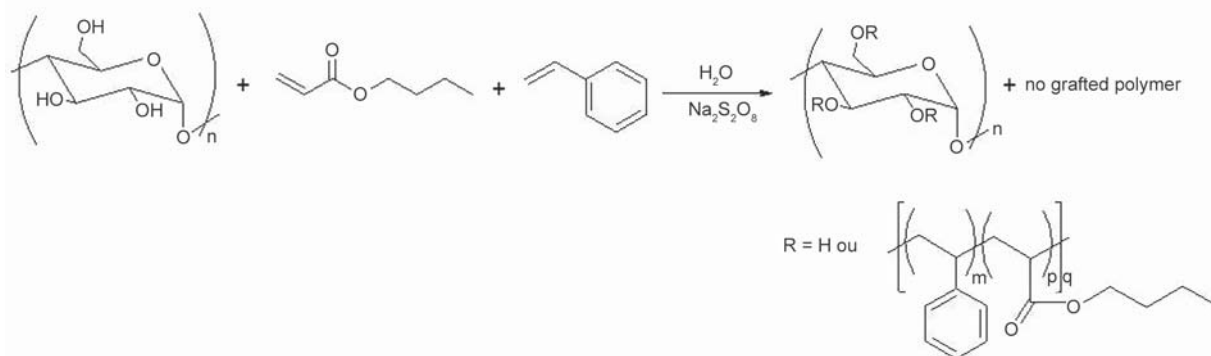
Figure 2. Grafting of poly(acrylate butyl- co -styrene) on dextrin/starch.
