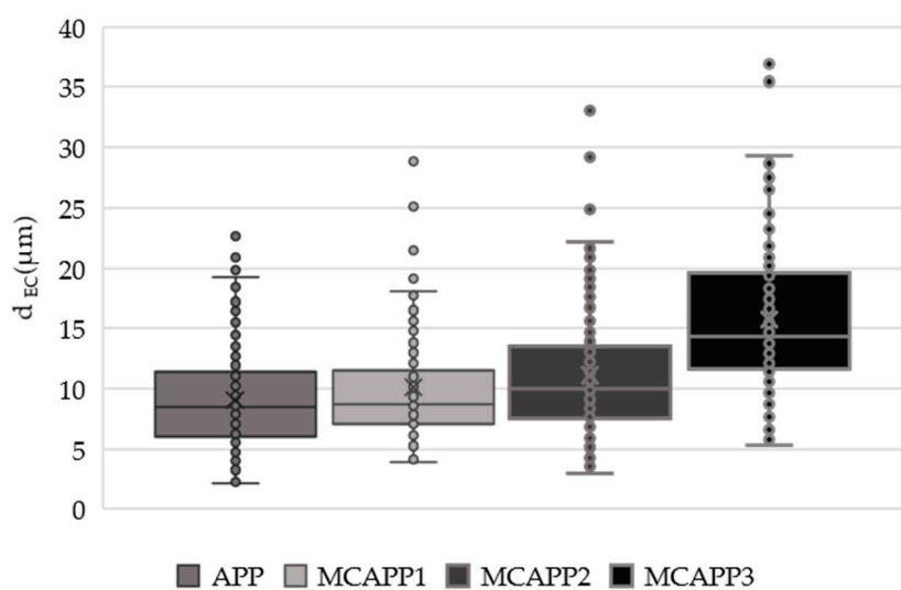
Figure 5. Box whiskers plot of the particles measured the diameter of a circle of equal projection area.
