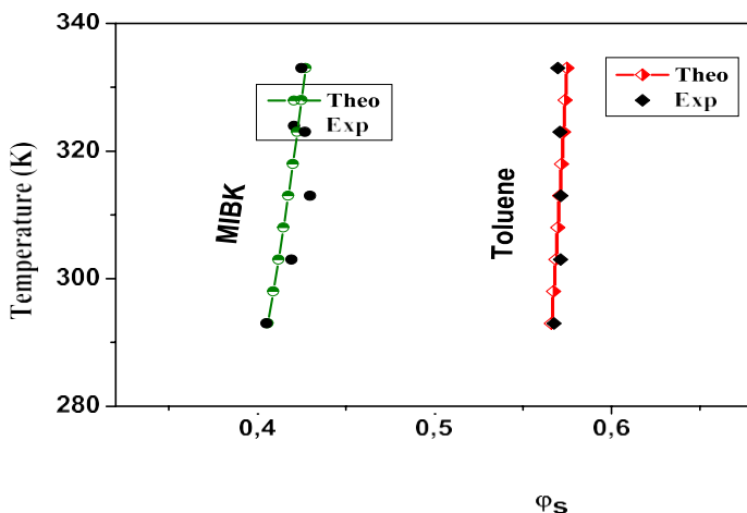
Fig. 20 Phase diagrams experimental and theoretical of poly(PEA)/0.1wt% HDDDA/solvents
